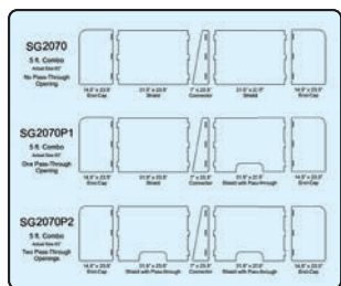
Diagram Of SG2070 Options
